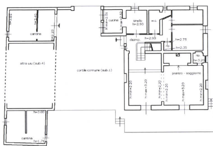
Piano Terreno
